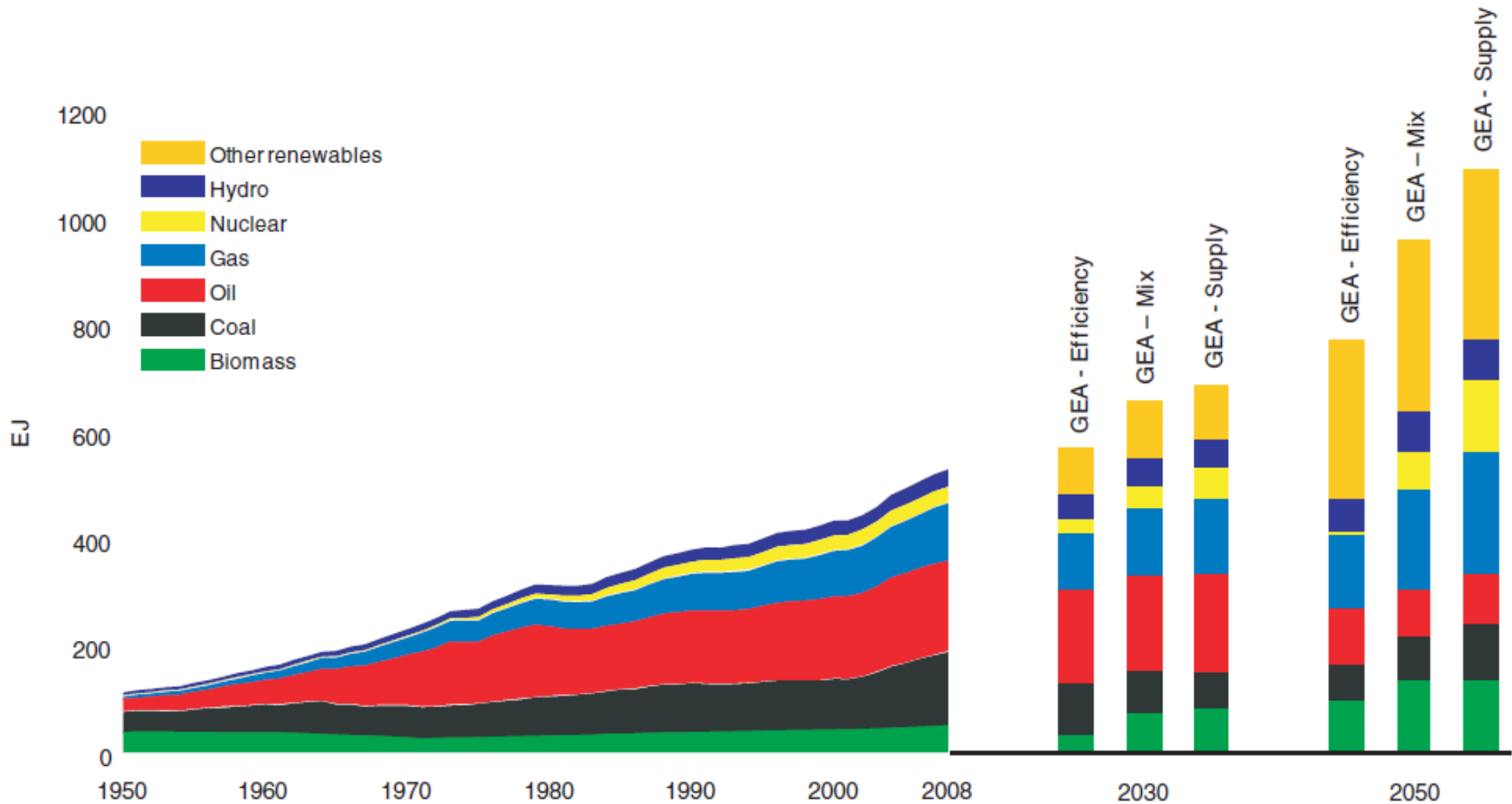
Figure SPM-3. | Development of primary energy to 2008 and in the three illustrative GEA pathways for the years 2030 and 2050. Source: based on Figures TS-24 and 17.13, Chapter 17. For further details of the GEA pathways see the interactive web-based GEA scenario database hosted by IIASA: www.iiasa.ac.at/web-apps/ene/geadb .
